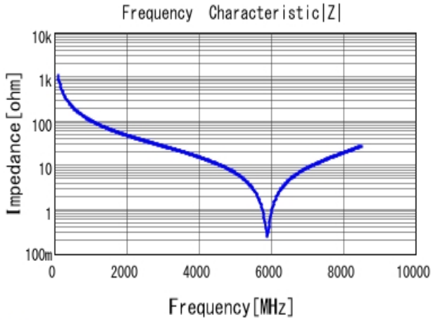
■ GQM1885C2A1R5BB01 |Z| DC0V, 25degC
