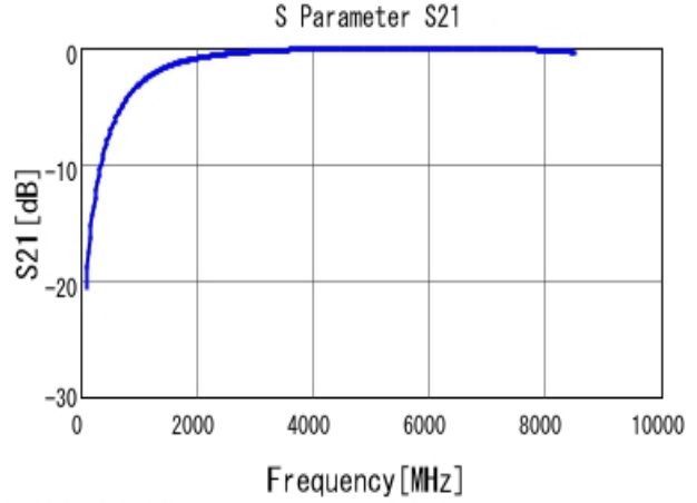
■ GQM1885C2A1R5BB01 S21 DCOV, 25degC
