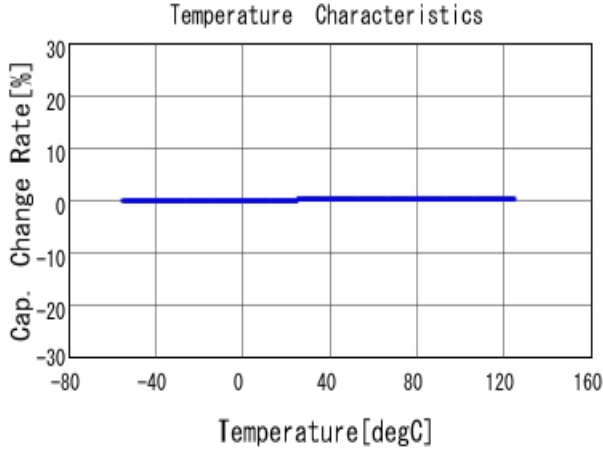
■ GQM1885C2A1R5BB01 C-Temp. capchange, DCOV, AC1Vrms
