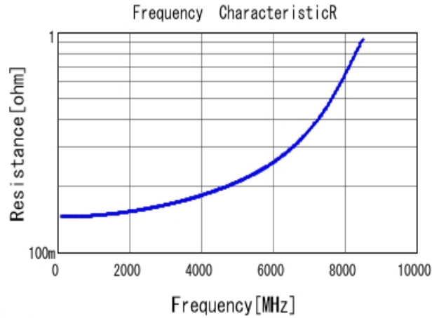
■ GQM1885C2A1R5BB01 R DC0V, 25degC
