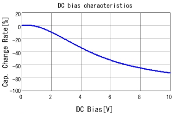
GGM155C71A105KE38 C-DC bias capchange, 25.0degC, A
