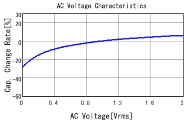
GGM155C71A105KE38 C-AC Voltage capchange, DCOV, 25
