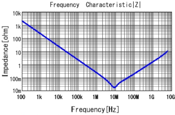
GGM155C71A105KE38 |Z| DCOV, 25degC
