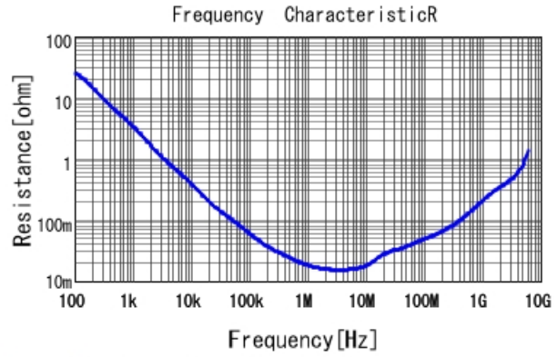
GGM155C71A105KE38 R DCOV, 25degC
