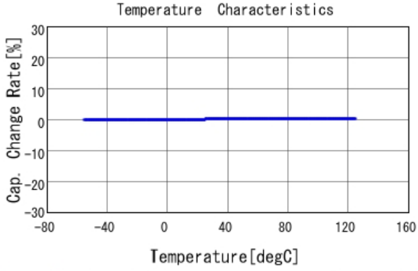
GRM1885C2A8R4DA01 C-Temp. capchange, DCOV, AC1Vrms
