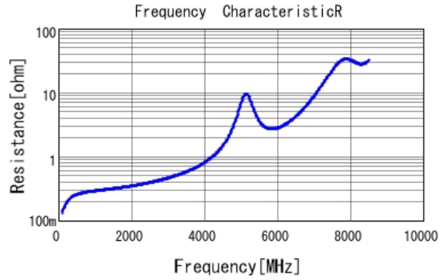
GRM1885C2A8R4DA01 R DCOV, 25degC
