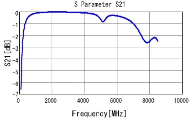
GRM1885C2A8R4DA01 S21 DCOV, 25degC
