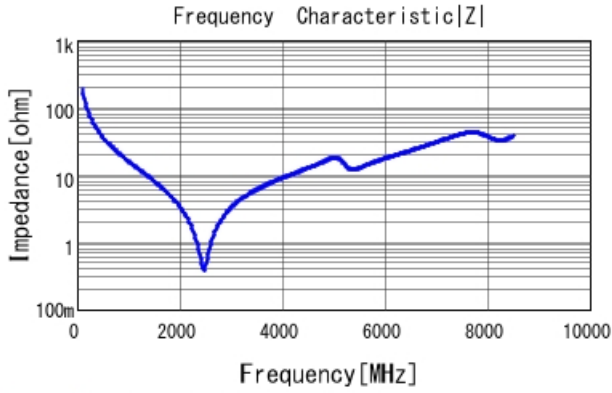
GRM1885C2A8R4DA01 |Z| DCOV, 25degC
