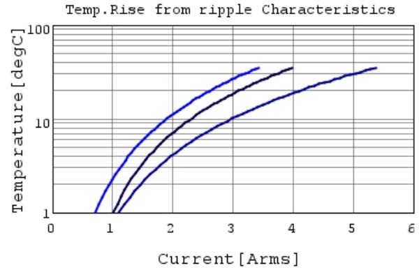
GCJ32DR72A225KA01 Temp.rise — 100kHz
