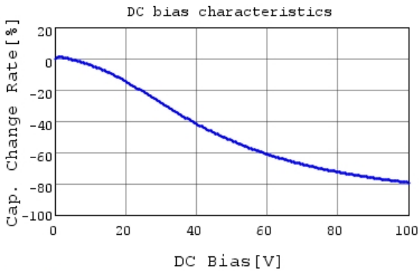
GCJ32DR72A225KA01 C-DC bias capchange, 25.0c
