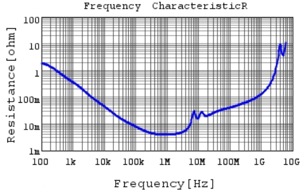
GCJ32DR72A225KA01 R DCOV, 25degC
