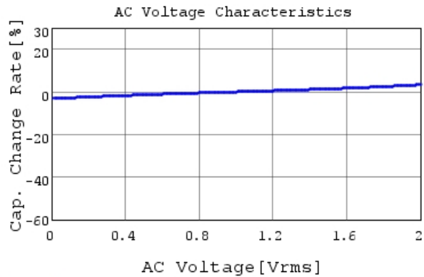
GCJ32DR72A225KA01 C-AC Voltage capchange, Dc
