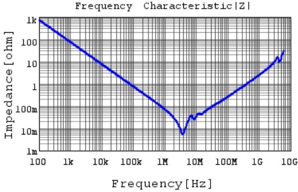
GCJ32DR72A225KA01 |Z| DCOV, 25degC
