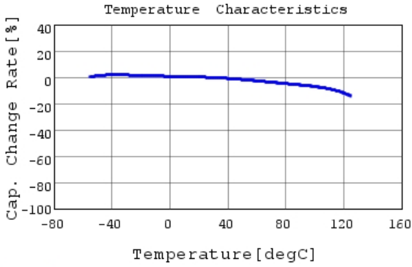
GCJ32DR72A225KA01 C-Temp. capchange, DC0.0V,
