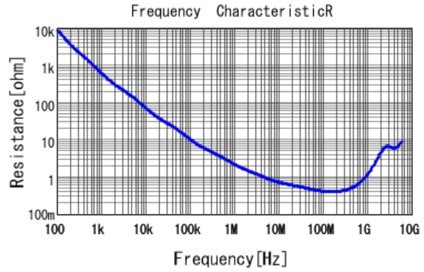
GCJ188R71E102KA01 R DCOV, 25degC
