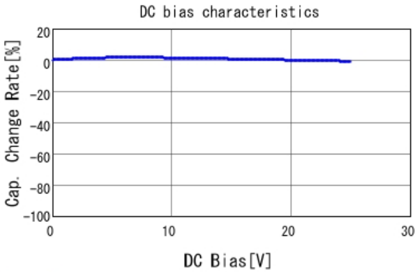
GCJ188R71E102KA01 C-DC bias capchange, 25.0degC, A
