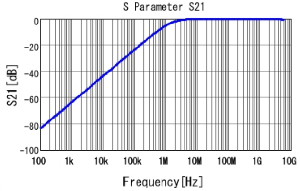
GCJ188R71E102KA01 S21 DC0V, 25degC
