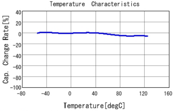
GCJ188R71E102KA01 C-Temp. capchange, DC0.0V, AC1.C
