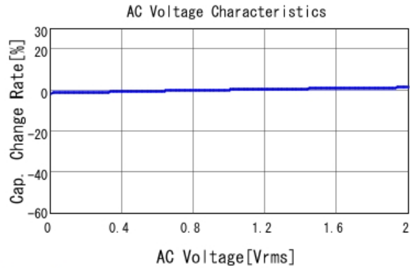
GCJ188R71E102KA01 C-AC Voltage capchange, DCOV, 25
