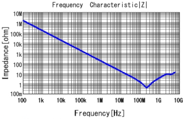
GCJ188R71E102KA01 |Z| DCOV, 25degC
