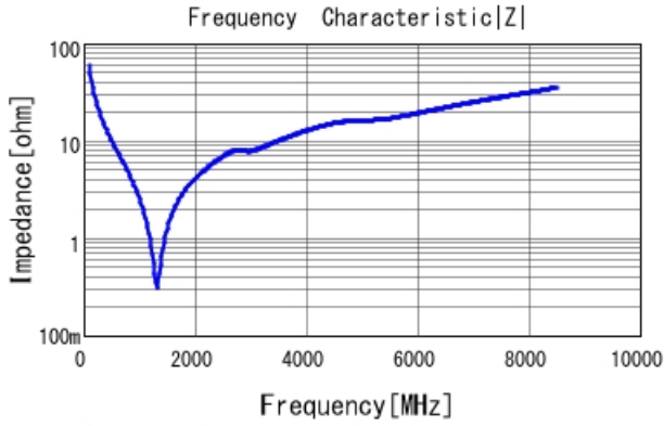
GRM1885C2A270JA01 |Z| DCOV, 25degC
