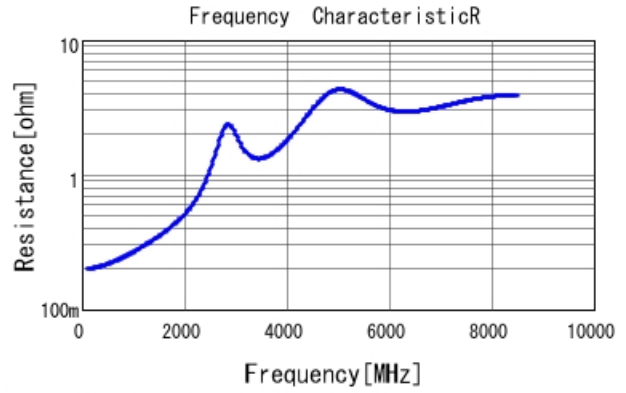
GRM1885C2A270JA01 R DCOV, 25degC
