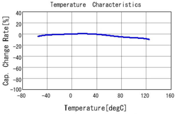
■ GCD188R71H822MA01 C-Temp. capchange, DCO. 0V, AC1. 0Vrm
