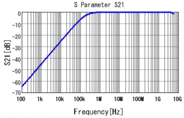
■ GCD188R71H822MA01 S21 DCOV, 25degC
