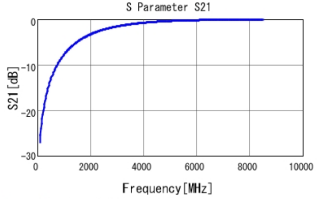
GRM1885C2AR70BA01 S21 DCOV, 25degC
