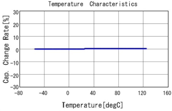
GRM1885C2AR70BA01 C-Temp. capchange, DCOV, AC1Vrms
