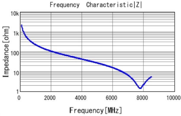
GRM1885C2AR70BA01 |Z| DCOV, 25degC
