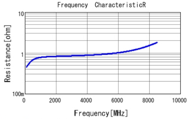
GRM1885C2AR70BA01 R DCOV, 25degC
