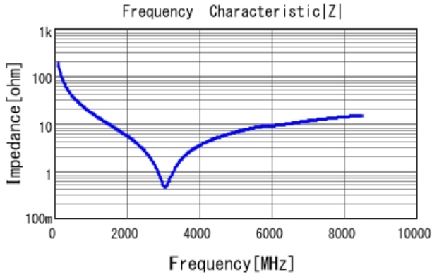
GRM1555C1H8R4BA01 |Z| DCOV, 25degC
