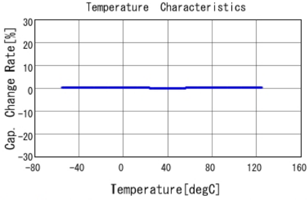
GRM1555C1H8R4BA01 C-Temp. capchange, DCOV, AC1Vrms
