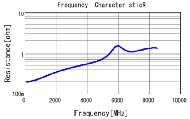
GRM1555C1H8R4BA01 R DCOV, 25degC
