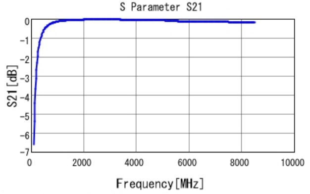
GRM1555C1H8R4BA01 S21 DCOV, 25degC
