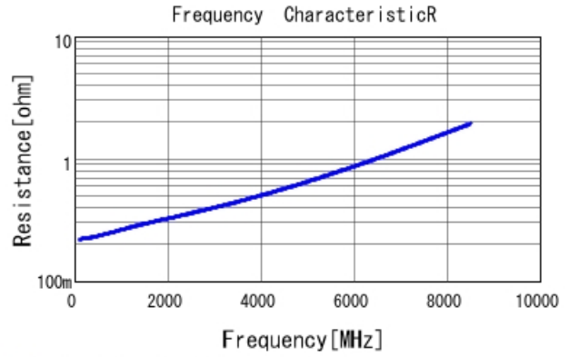
■ GRM0335C2A4R5BA01 R DC0V, 25degC
