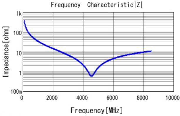
■ GRM0335C2A4R5BA01 |Z| DC0V, 25degC
