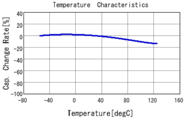
GGM155R71H104KE02 C-Temp. capchange, DC0.0V, AC1.C
