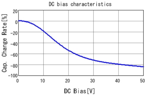
GGM155R71H104KE02 C-DC bias capchange, 25.0degC, A
