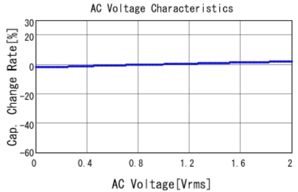
RCER71H473K0A2H03B C-AC Voltage capchange, DC0V, 2
