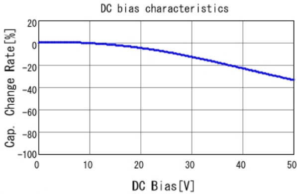
RCER71H473K0A2H03B C-DC bias capchange, 25.0degC,
