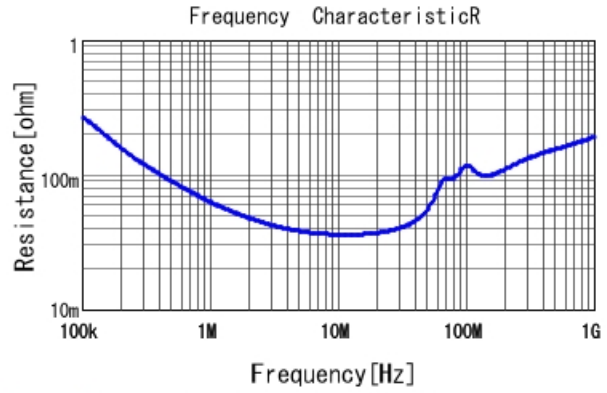
RCER71H473K0A2H03B R DC0V, 25degC
