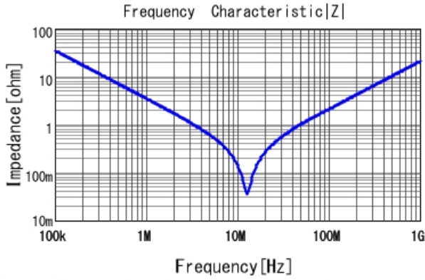
RCER71H473K0A2H03B |Z| DC0V, 25degC
