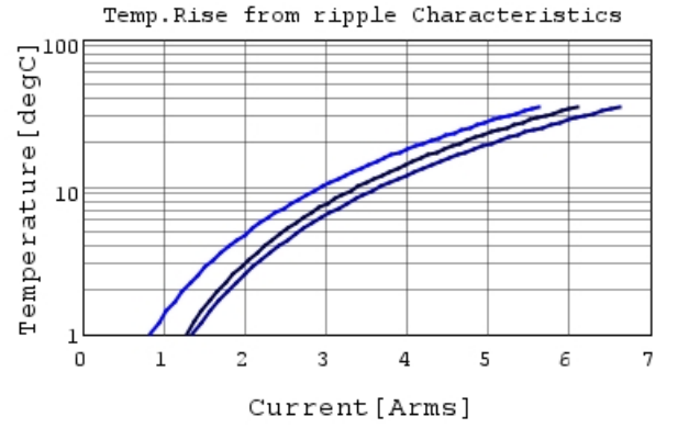
GRM31CR61A476KE15 Temp.rise — 60kHz —
