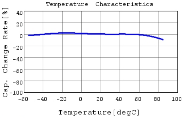
GRM31CR61A476KE15 C-Temp. capchange, DC0.0V,
