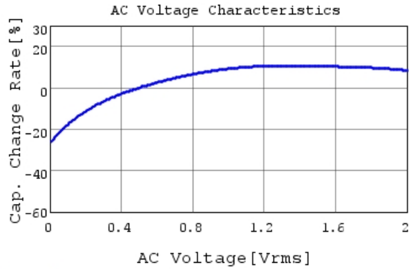
GRM31CR61A476KE15 C-AC Voltage capchange, Dc
