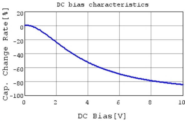
GRM31CR61A476KE15 C-DC bias capchange, 25.0c
