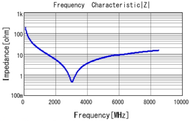
GRM1555C1H8R5CA01 |Z| DCOV, 25degC
