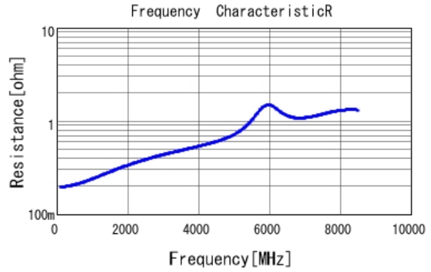
GRM1555C1H8R5CA01 R DCOV, 25degC
