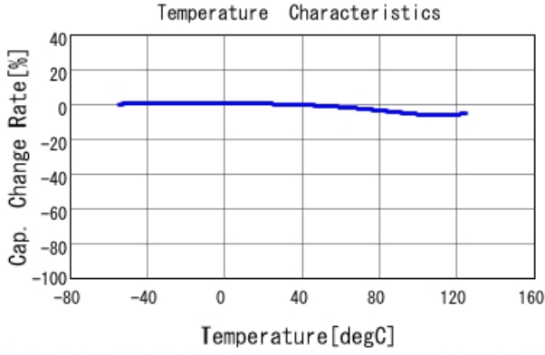
■ GRM033R71H102MA12 C-Temp. capchange, DCO. 0V, AC1. 0Vrm
