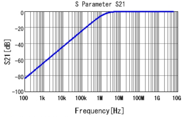
■ GRM033R71H102MA12 S21 DCOV, 25degC
