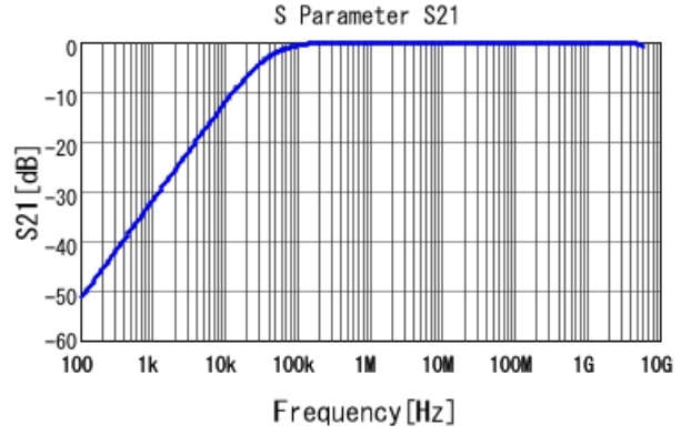
■ GCE188R71E393KA01 S21 DCOV, 25degC
