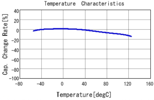
■ GCE188R71E393KA01 C-Temp. capchange, DCO. 0V, AC1. 0Vrm
