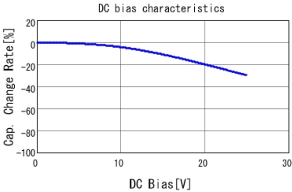
■ GCE188R71E393KA01 C-DC bias capchange, 25.0degC, AC1.
