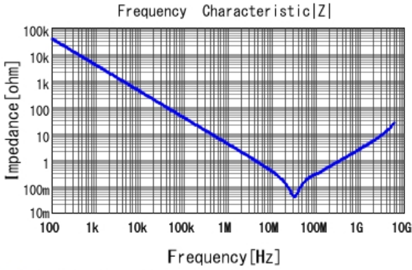
■ GCE188R71E393KA01 |Z| DC0V, 25degC
