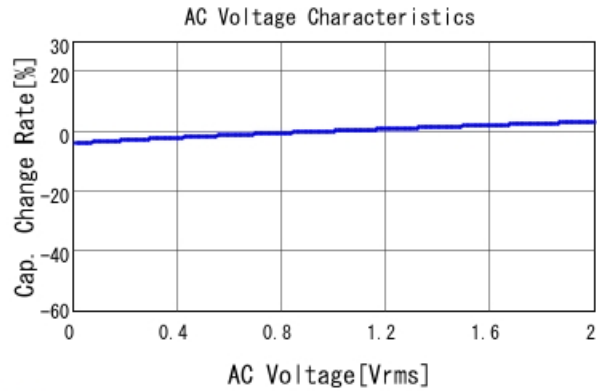
■ GCE188R71E393KA01 C-AC Voltage capchange, DC0V, 25.0d
