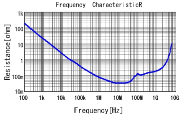
■ GCE188R71E393KA01 R DC0V, 25degC
