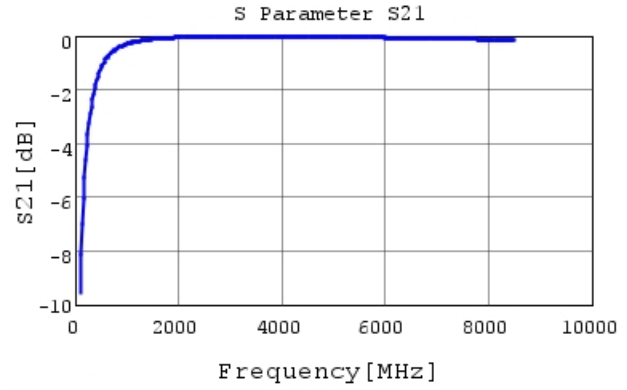
GCQ1555C1H5R6BB01 S21 DCOV, 25degC
