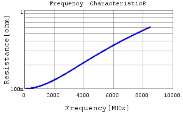
GCQ1555C1H5R6BB01 R DC0V, 25degC
