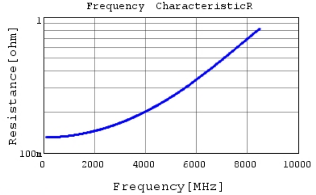
GCQ1555C1H3R6BB01 R DC0V, 25degC
