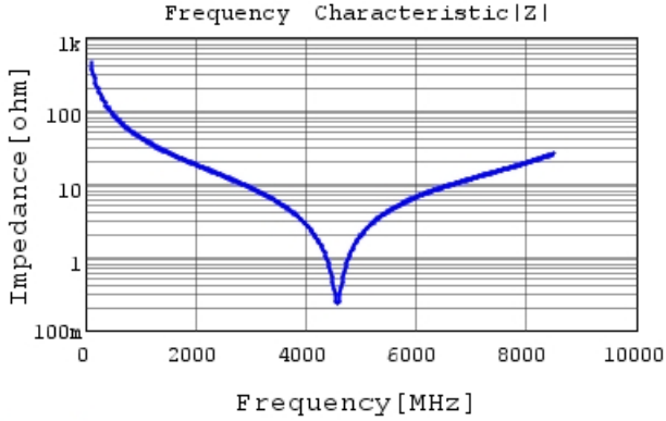
GCQ1555C1H3R6BB01 |Z| DC0V, 25degC
