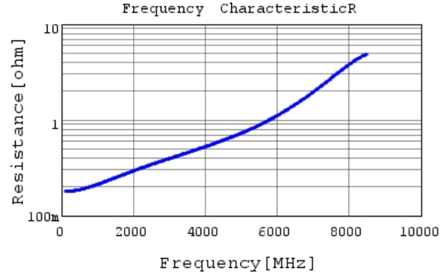
GRM0332C2A150JA01 R DCOV, 20degC
