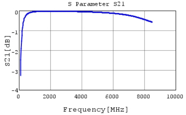
GRM0332C2A150JA01 S21 DCOV, 20degC
