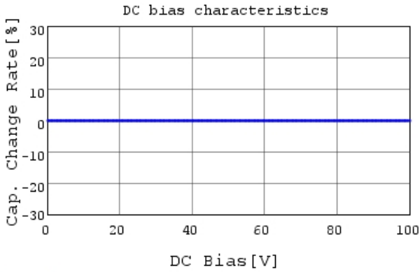
GRM0332C2A150JA01 C-DC bias capchange, 20.0c
