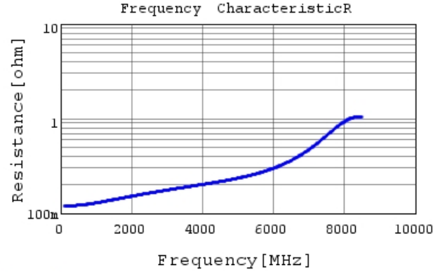
GCQ1555C1H4R5BB01 R DC0V, 25degC
