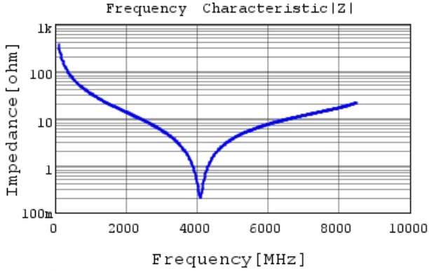
GCQ1555C1H4R5BB01 |Z| DC0V, 25degC
