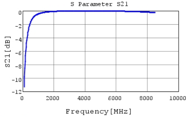
GCQ1555C1H4R5BB01 S21 DCOV, 25degC
