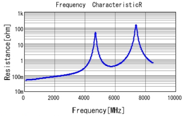
GQM1875C2E150JB12 R DCOV, 25degC
