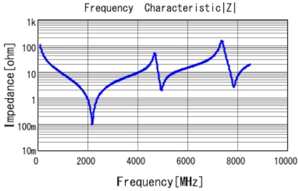
GQM1875C2E150JB12 |Z| DCOV, 25degC
