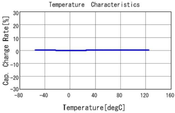
GQM1875C2E150JB12 C-Temp. capchange, DCOV, AC1Vrms
