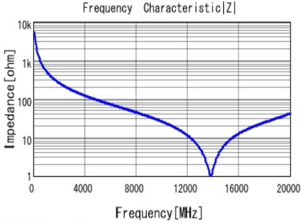
■ GRM1555C1HR30BA01 |Z| DCOV, 25degC
