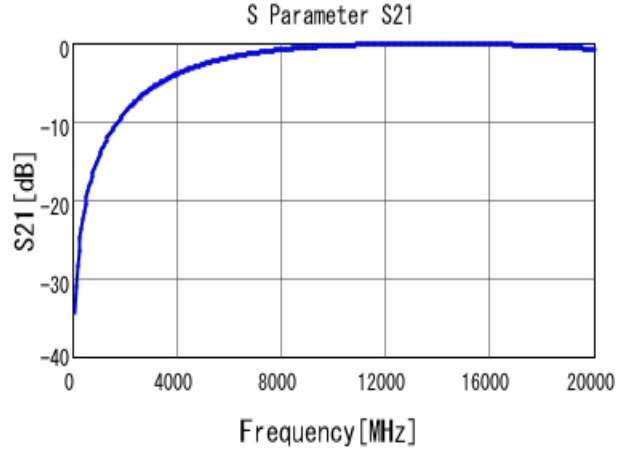
■ GRM1555C1HR30BA01 S21 DCOV, 25degC
