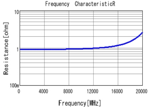
■ GRM1555C1HR30BA01 R DCOV, 25degC
