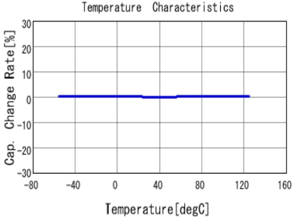
■ GRM1555C1HR30BA01 C-Temp. capchange, DCOV, AC1Vrms
