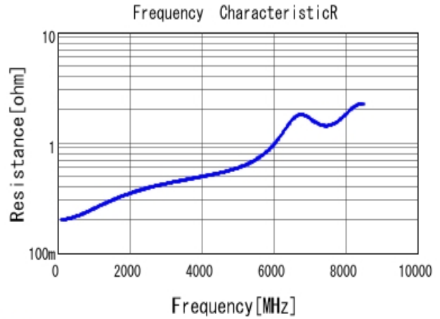
■ GRM1555C1H6R8BA01 R DCOV, 25degC
