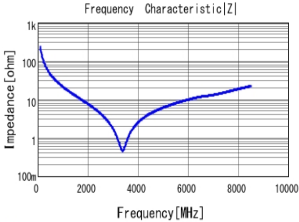
■ GRM1555C1H6R8BA01 |Z| DCOV, 25degC
