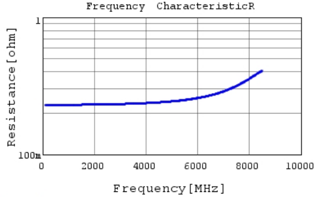
GCQ1555C1H1R3BB01 R DC0V, 25degC
