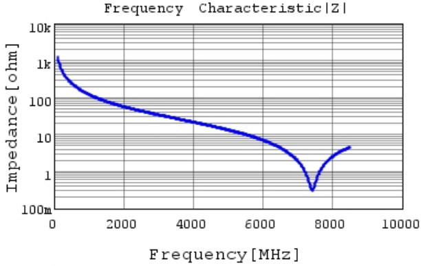
GCQ1555C1H1R3BB01 |Z| DC0V, 25degC
