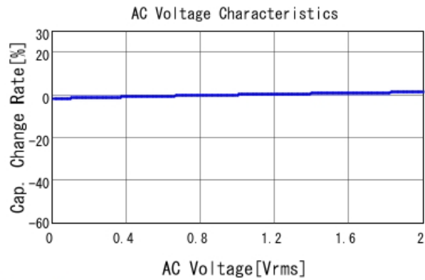
GCJ188R71E392KA01 C-AC Voltage capchange, DCOV, 25
