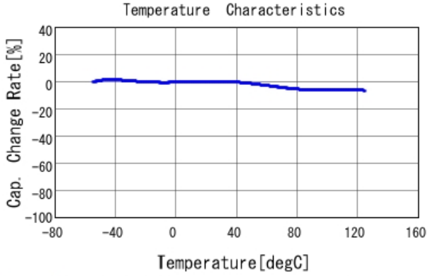
GCJ188R71E392KA01 C-Temp. capchange, DC0.0V, AC1.C
