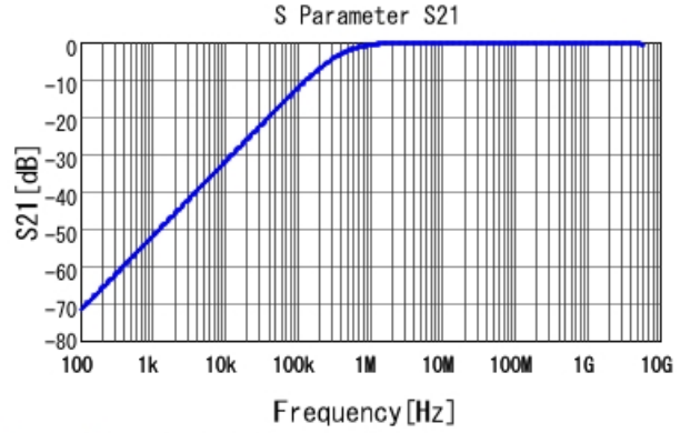
GCJ188R71E392KA01 S21 DC0V, 25degC
