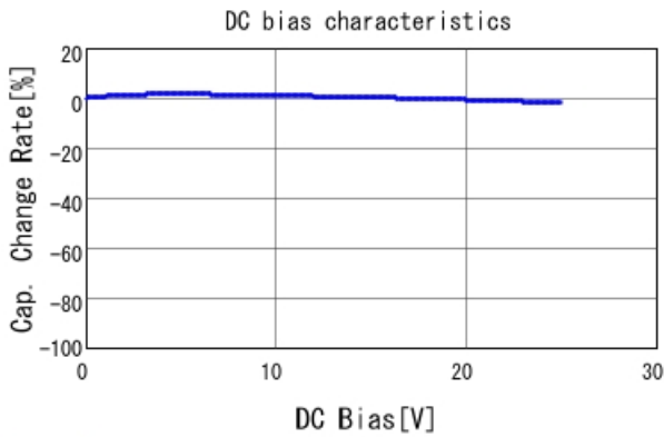
GCJ188R71E392KA01 C-DC bias capchange, 25.0degC, A
