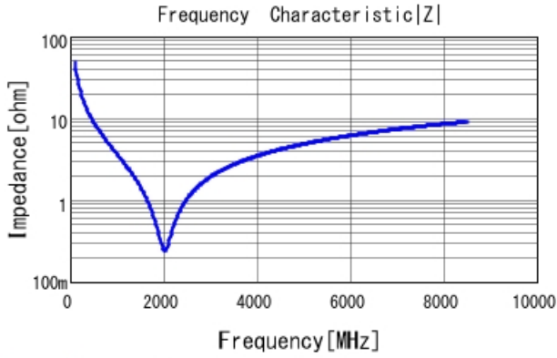
GRM0225C1C330JA02 |Z| DCOV, 25degC
