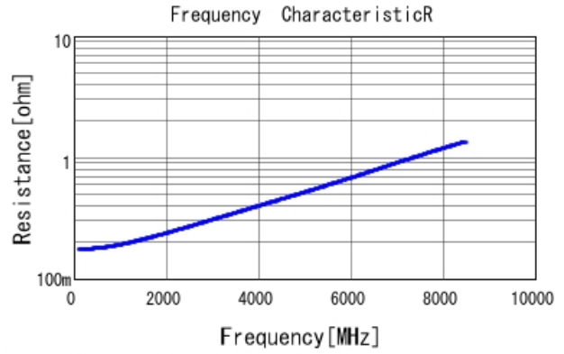
GRM0225C1C330JA02 R DCOV, 25degC
