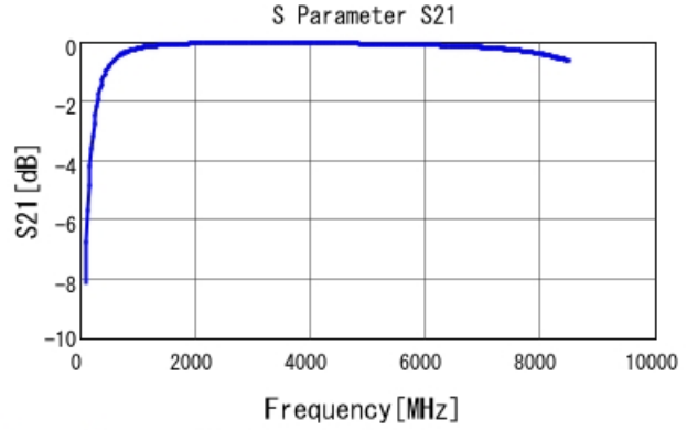
GRM0335C1H6R8CA01 S21 DCOV, 25degC
