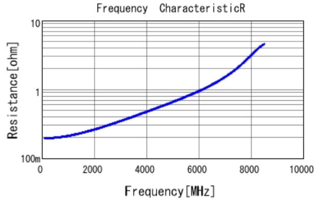
GRM0335C1H6R8CA01 R DCOV, 25degC
