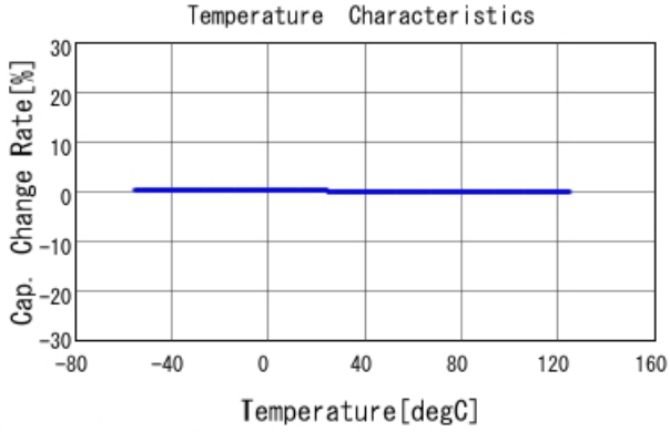
GRM0335C1H6R8CA01 C-Temp. capchange, DCOV, AC1Vrms
