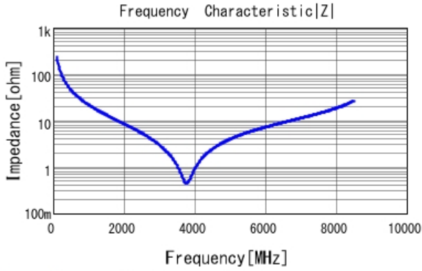
GRM0335C1H6R8CA01 |Z| DCOV, 25degC
