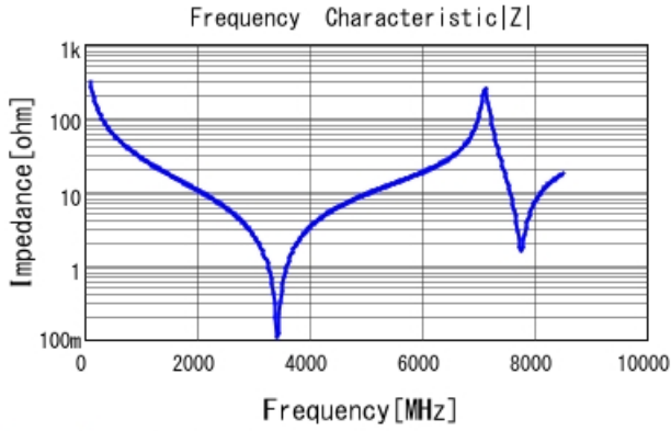
GQM2195G2E5R1CB12 |Z| DCOV, 25degC
