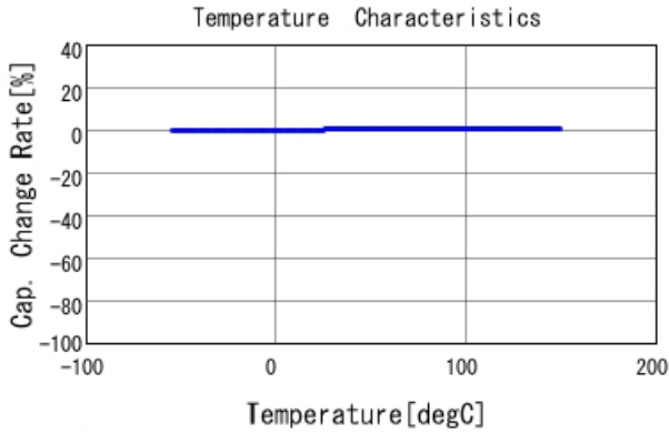
GQM2195G2E5R1CB12 C-Temp. capchange, DCOV, AC1Vrms
