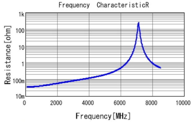
GQM2195G2E5R1CB12 R DCOV, 25degC
