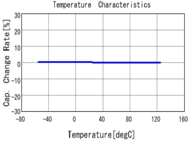
■ GRM1885C1H561JA01 C-Temp. capchange, DCOV, AC1Vrms
