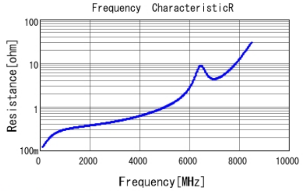
GRM1885C1H6R4CA01 R DCOV, 25degC
