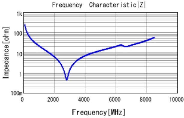
GRM1885C1H6R4CA01 |Z| DCOV, 25degC
