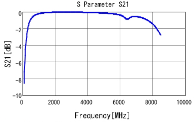
GRM1885C1H6R4CA01 S21 DCOV, 25degC
