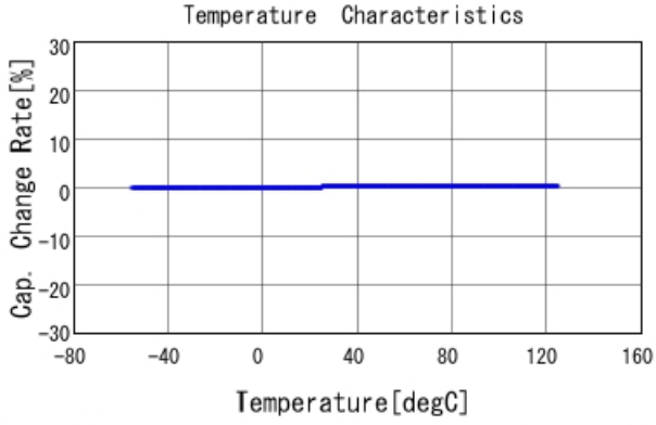
GRM1885C1H6R4CA01 C-Temp. capchange, DCOV, AC1Vrms
