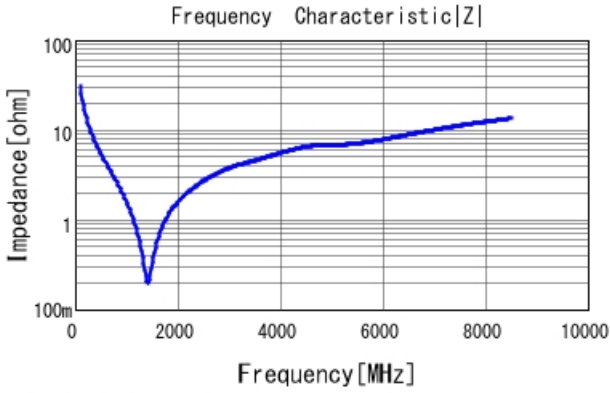
■ GRM0335C1H510JA01 |Z| DCOV, 25degC
