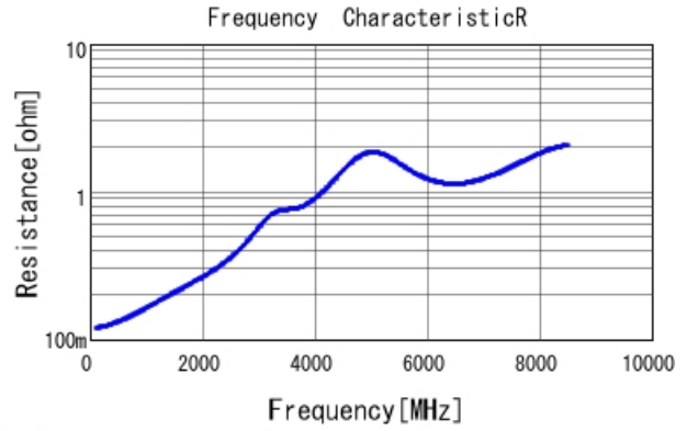
■ GRM0335C1H510JA01 R DCOV, 25degC
