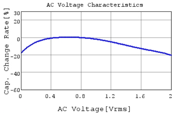
GRM033R60J225ME15 C-AC Voltage capchange, Dc
