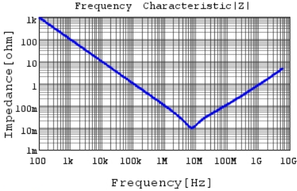
GRM033R60J225ME15 |Z| DCOV, 25degC
