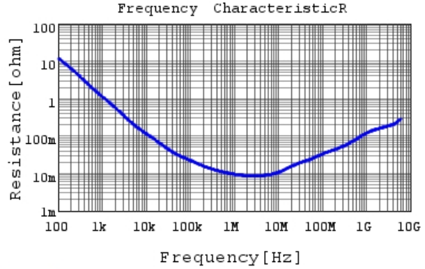
GRM033R60J225ME15 R DCOV, 25degC
