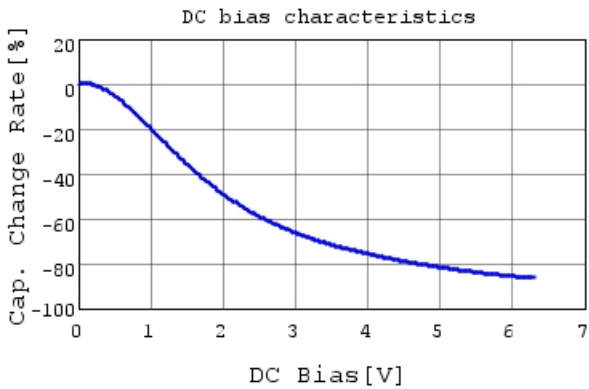
GRM033R60J225ME15 C-DC bias capchange, 25.0c
