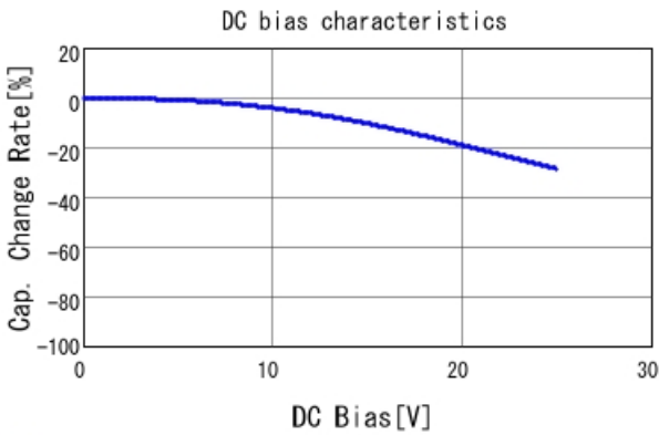
■ GCE188R71E473MA01 C-DC bias capchange, 25.0degC, AC1.
