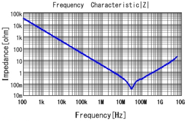
■ GCE188R71E473MA01 |Z| DCOV, 25degC
