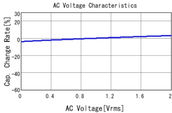
■ GCE188R71E473MA01 C-AC Voltage capchange, DCOV, 25.0d
