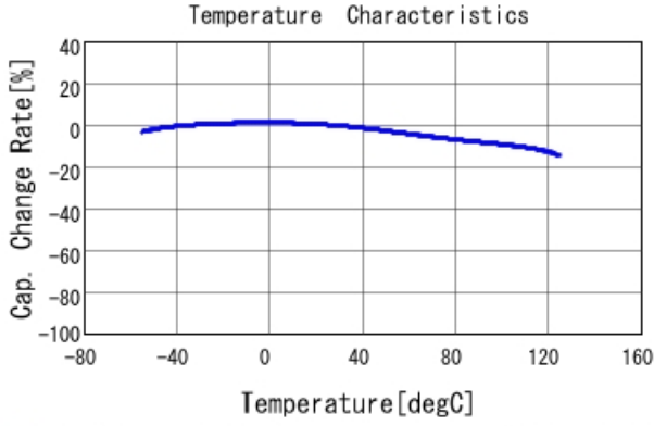
■ GCE188R71E473MA01 C-Temp. capchange, DCO. 0V, AC1. 0Vrm
