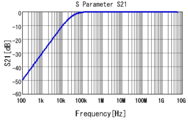
■ GCE188R71E473MA01 S21 DCOV, 25degC
