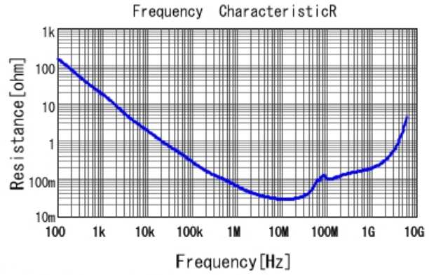
■ GCE188R71E473MA01 R DCOV, 25degC
