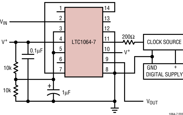
Figure 3. Single Supply Operation for an f_{\text{CLK}}/f_{\text{CUTOFF}} = 50:1
