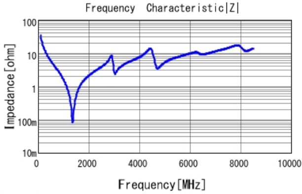
GJM1555C1H470JB01 |Z| DCOV, 25degC
