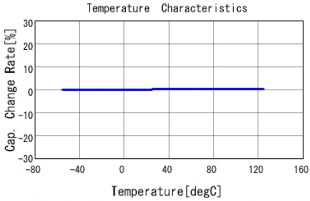
GJM1555C1H470JB01 C-Temp. capchange, DCOV, AC1Vrms
