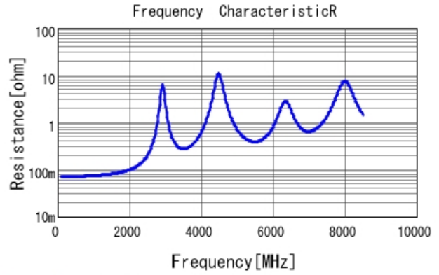
GJM1555C1H470JB01 R DCOV, 25degC
