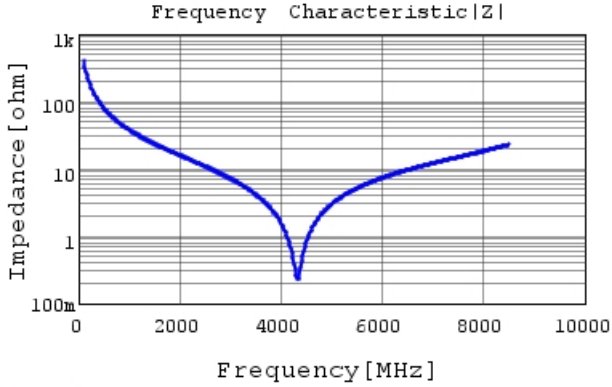
GCQ1555C1H4R0BB01 |Z| DC0V, 25degC
