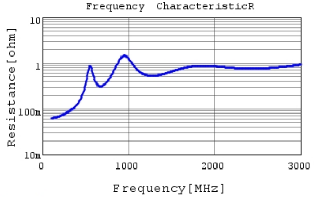
GRM31B5C2J681FW01 R DC0V, 25degC
