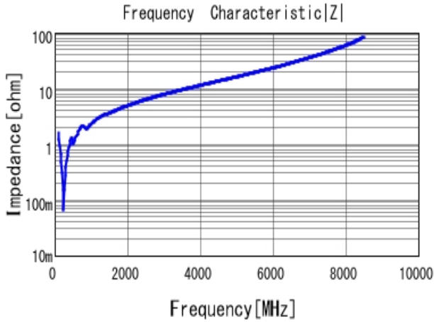
■ GRT1885C2A821JA02 |Z| DCOV, 25degC
