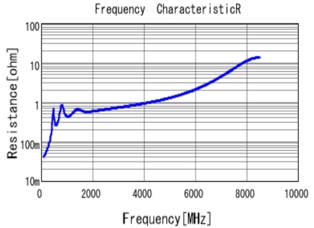
■ GRT1885C2A821JA02 R DCOV, 25degC
