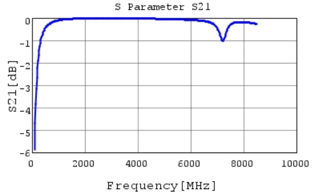
GCQ1555C1H9R4BB01 S21 DCOV, 25degC
