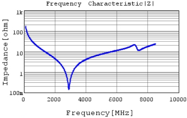
GCQ1555C1H9R4BB01 |Z| DC0V, 25degC
