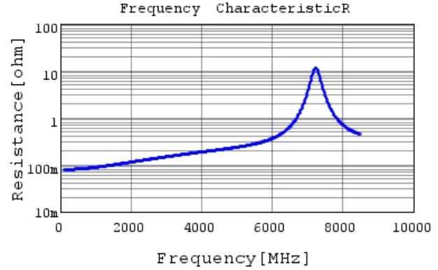
GCQ1555C1H9R4BB01 R DC0V, 25degC
