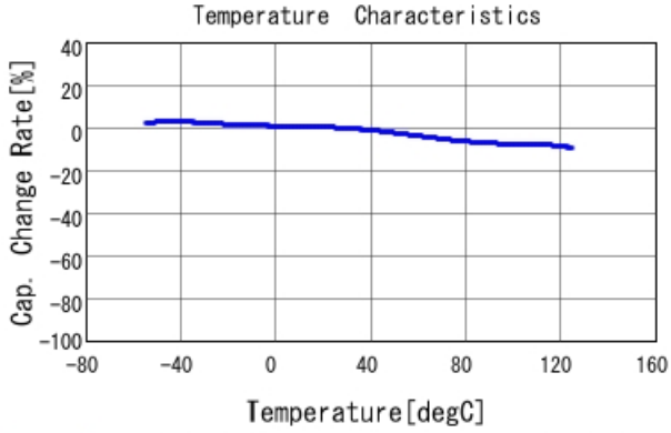
GCM033R71C182KA55 C-Temp. capchange, DC0.0V, AC1.C
