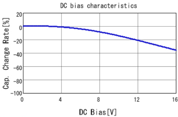
GCM033R71C182KA55 C-DC bias capchange, 25.0degC, A
