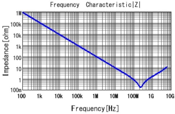
GCM033R71C182KA55 |Z| DCOV, 25degC
