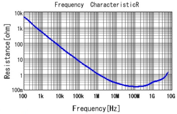
GCM033R71C182KA55 R DCOV, 25degC
