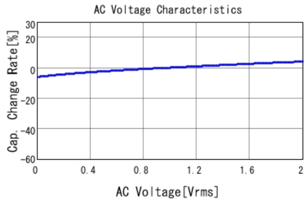
GCM033R71C182KA55 C-AC Voltage capchange, DCOV, 25
