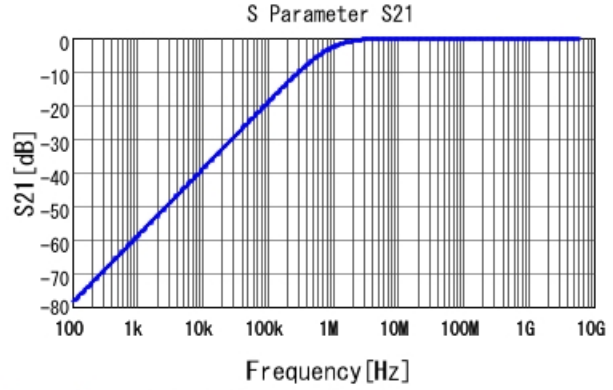
GCM033R71C182KA55 S21 DC0V, 25degC
