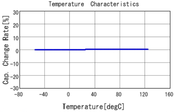
GRM1885C2A5R8BA01 C-Temp. capchange, DC0V, AC1Vrms
