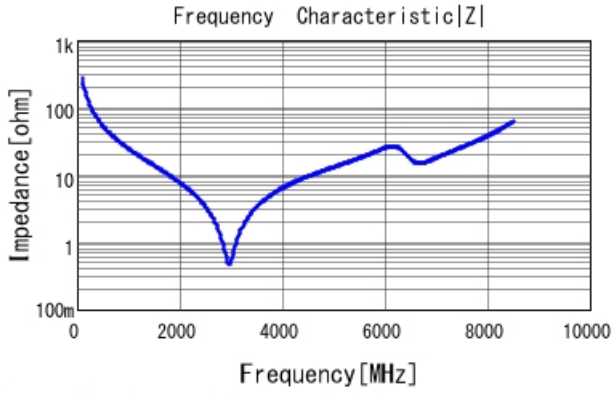
GRM1885C2A5R8BA01 |Z| DCOV, 25degC
