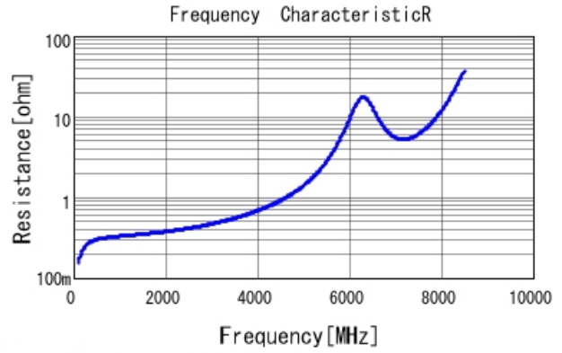
GRM1885C2A5R8BA01 R DCOV, 25degC
