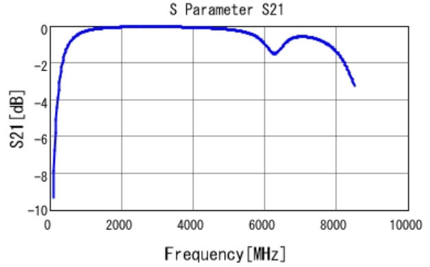
GRM1885C2A5R8BA01 S21 DC0V, 25degC
