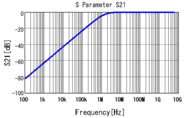
■ GCD188R72A122KA01 S21 DCOV, 25degC
