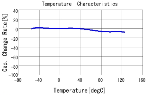
■ GCD188R72A122KA01 C-Temp. capchange, DCO. 0V, AC1. 0Vrm
