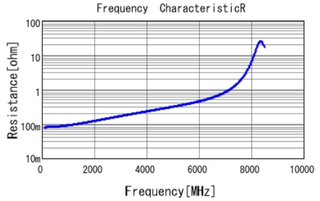
GJM1555C1H7R5CB01 R DCOV, 25degC
