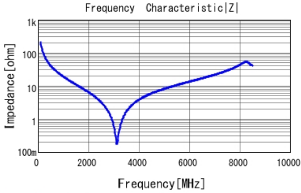
GJM1555C1H7R5CB01 |Z| DCOV, 25degC
