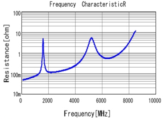
■ GQM1885C1H680JB01 R DC0V, 25degC
