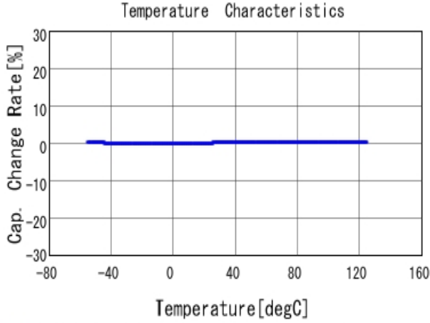
■ GQM1885C1H680JB01 C-Temp. capchange, DCOV, AC1Vrms
