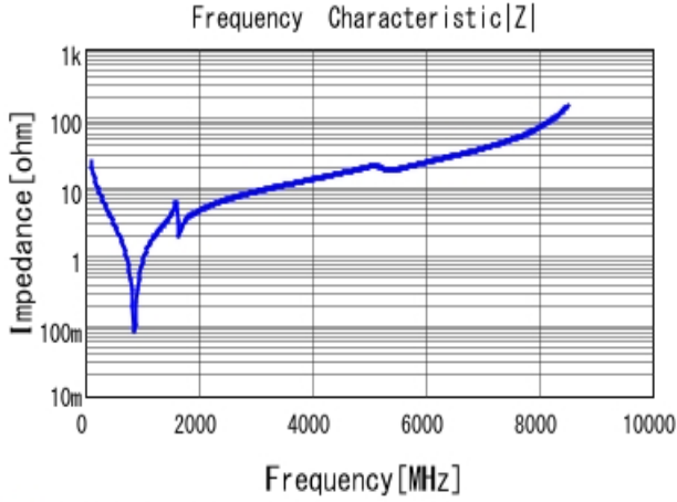
■ GQM1885C1H680JB01 |Z| DC0V, 25degC
