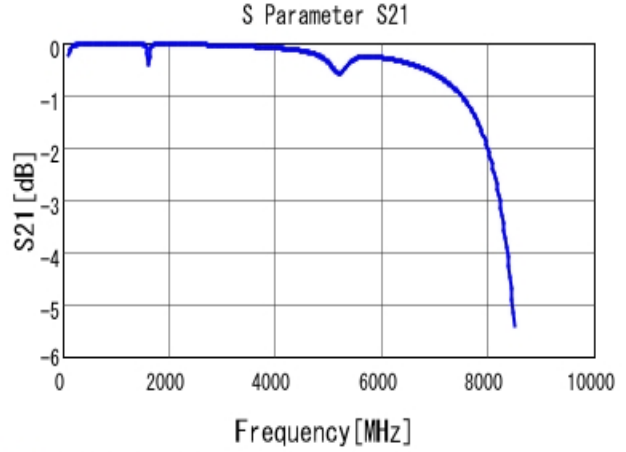
■ GQM1885C1H680JB01 S21 DCOV, 25degC
