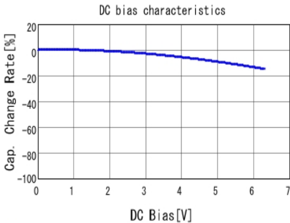
■ GRM033R10J682KA01 C-DC bias capchange, 20.0degC, AC1.
