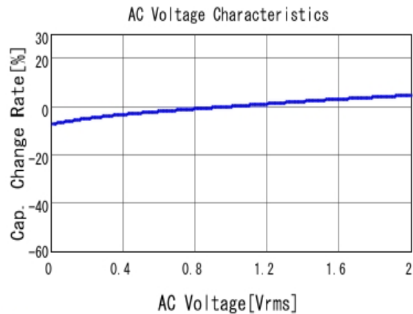
■ GRM033R10J682KA01 C-AC Voltage capchange, DC0V, 20.0d
