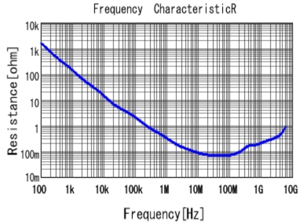
■ GRM033R10J682KA01 R DC0V, 20degC
