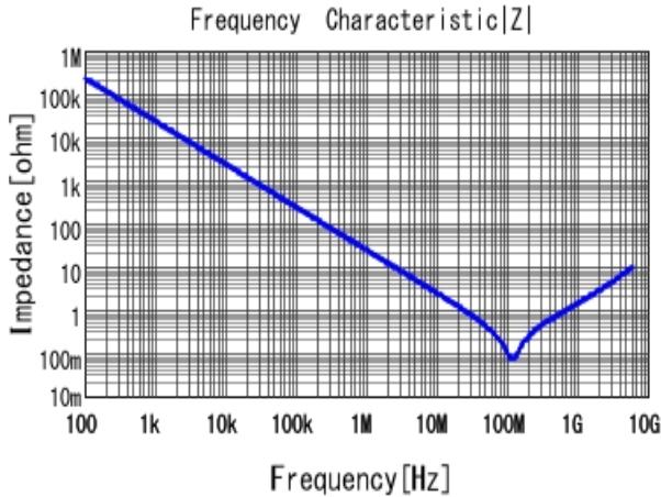
■ GRM033R10J682KA01 |Z| DC0V, 20degC
