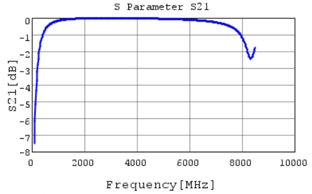
GCQ1555C1H7R4CB01 S21 DCOV, 25degC
