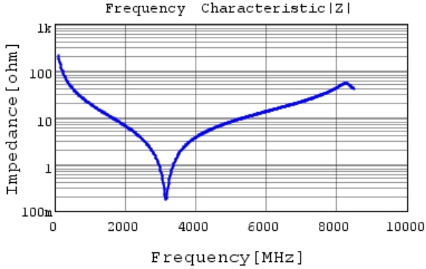
GCQ1555C1H7R4CB01 |Z| DC0V, 25degC
