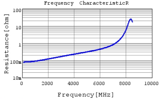
GCQ1555C1H7R4CB01 R DC0V, 25degC
