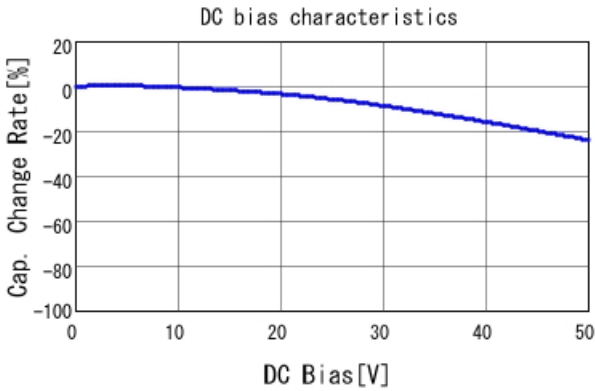
GCD21BR71H333KA01 C-DC bias capchange, 25.0degC, A
