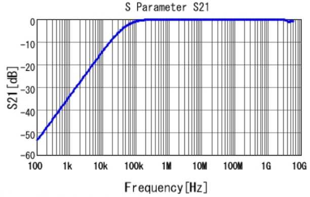
GCD21BR71H333KA01 S21 DC0V, 25degC
