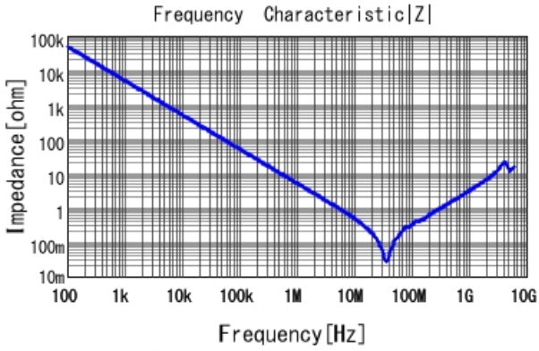
GCD21BR71H333KA01 |Z| DCOV, 25degC
