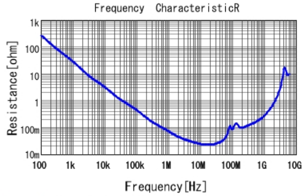
GCD21BR71H333KA01 R DCOV, 25degC
