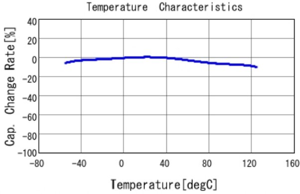
GCD21BR71H333KA01 C-Temp. capchange, DC0.0V, AC1.C
