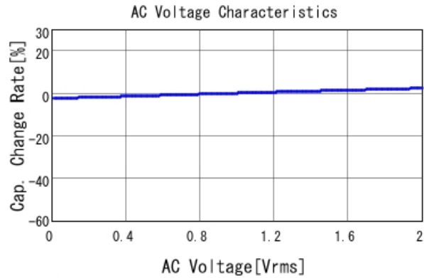
GCD21BR71H333KA01 C-AC Voltage capchange, DCOV, 25
