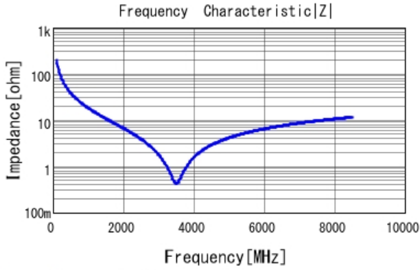
GRM0335C1H8R0BA01 |Z| DCOV, 25degC
