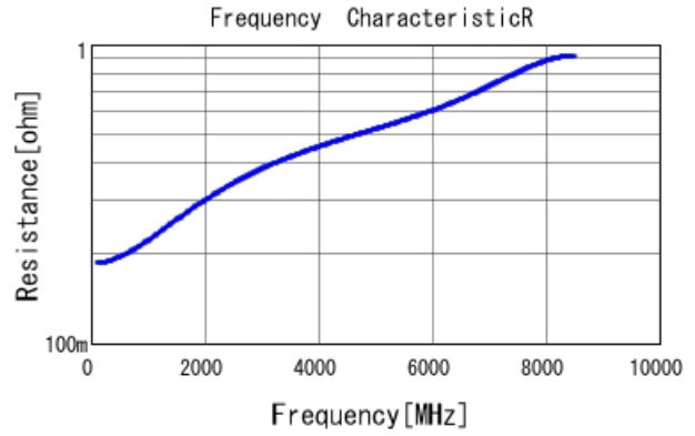
GRM0335C1H8R0BA01 R DCOV, 25degC
