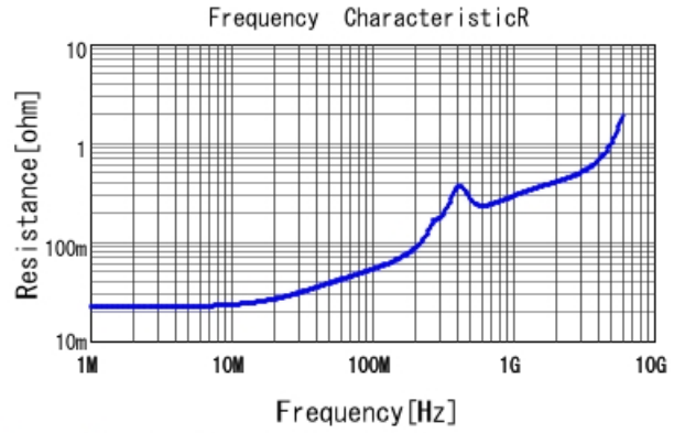
GRM1887U1H272JA01 R DCOV, 25degC
