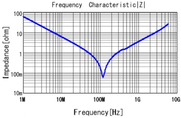
GRM1887U1H272JA01 |Z| DCOV, 25degC
