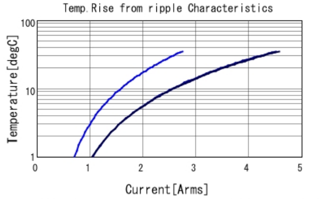
GRM21BR61A225MA01 Temp. rise — 100kHz — 500
