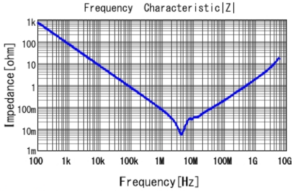
GRM21BR61A225MA01 |Z| DCOV, 25degC
