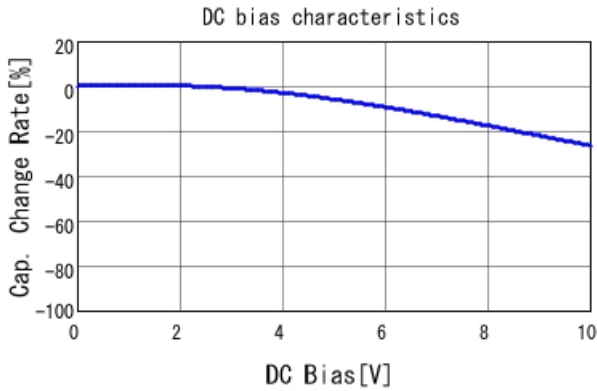
GRM21BR61A225MA01 C-DC bias capchange, 25.0degC, A
