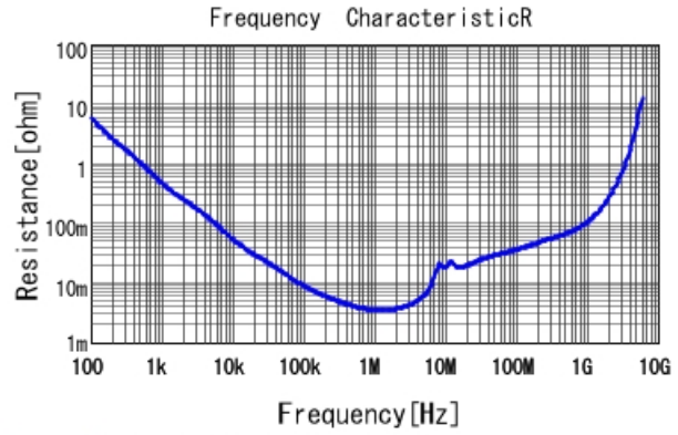
GRM21BR61A225MA01 R DCOV, 25degC
