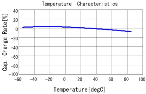
GRM21BR61A225MA01 C-Temp. capchange, DC0.0V, AC1.C
